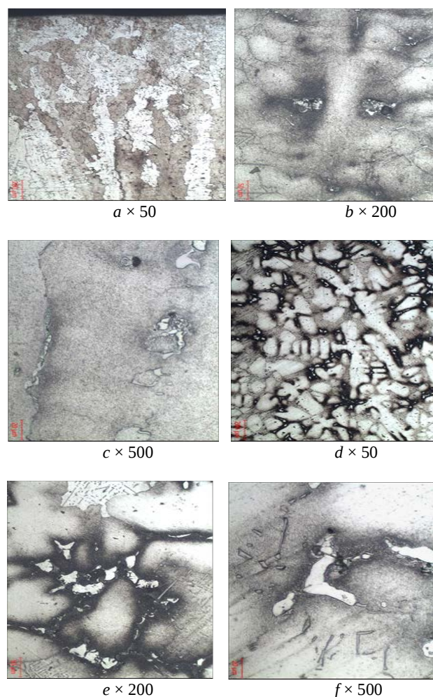
Figure 2. Microstructure in the edge ( a , b , c ) and central ( d , e , f ) zones of sample 1
